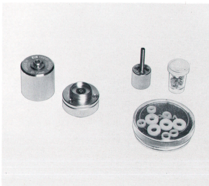
Fig. 10. 16091A coaxial fixture set consists of cavity-type fixtures useful up to 1000 MHz.
