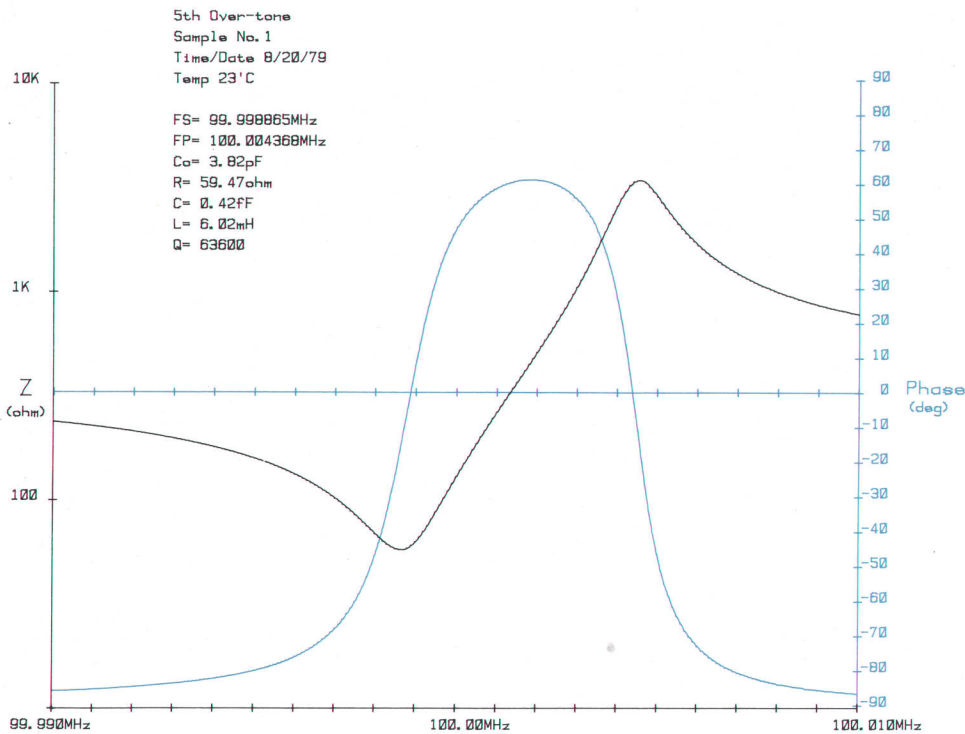
Fig. 3. |Z| - \Theta characteristics of a 100-MHz fifth-overtone quartz crystal.
