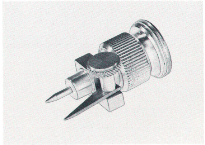
Fig. 13. 16094A probe fixture, mounted at the tip of a precision coaxial cable, is useful to 125 MHz.
