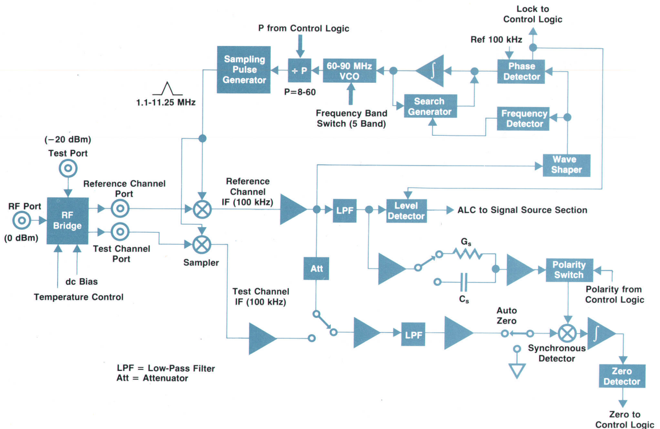
Fig. 7. 4191A receiver section down-converts and detects the test and reference signals from the RF bridge, and measures the vector ratio of these signals to determine the reflection coefficient of the device under test.
